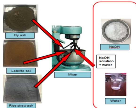
Figure 1. Mixing geopolymer.
